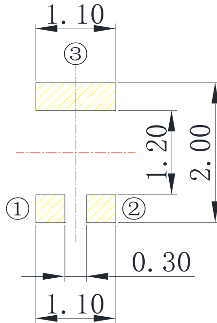
Figure 3. Recommended landing pattern on customers' PCB
